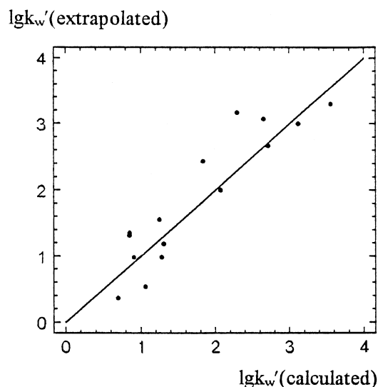
Figure 1. Plot of extrapolated and the calculated \log k_w' values according to Eq. 3.
