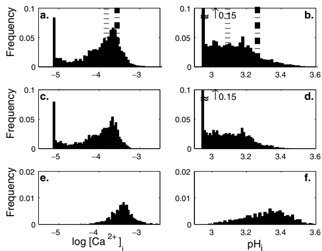
Fig. 4. Steady-state distributions of \log[\text{Ca}^{2+}] and \text{pH} in all pores (a and b); in non-reactive pores (c and d), and in reactive pores (e and f). The dot-dashed lines indicate the uniform concentrations from the continuum model. The dotted lines indicate the volume-averaged concentrations.
