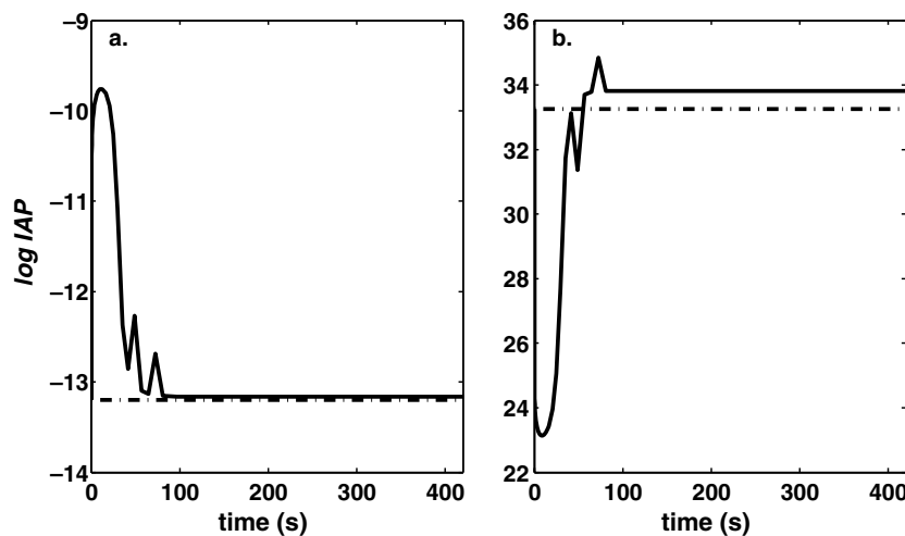
Fig. 10. Evolution of \log IAP for case A: (a) water dissociation reaction H_2O = H^+ + OH^- ; (b) Al^{3+} speciation reaction Al^{3+} + 4OH^- = Al(OH)_4^- . The dashed lines indicate the value of \log K_{eq} for each reaction.
