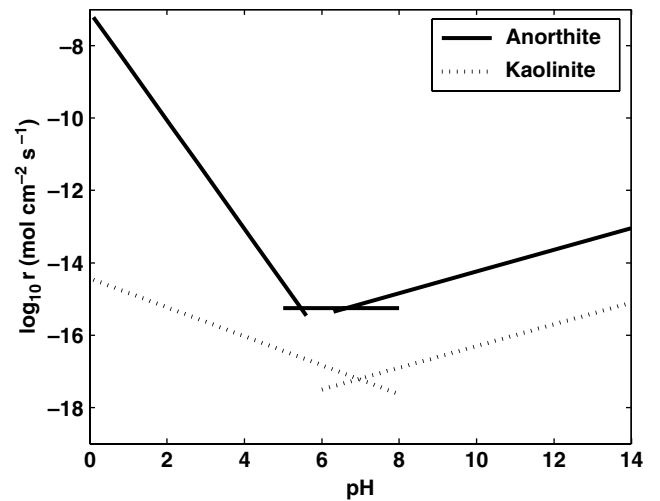
Fig. 1. Dissolution rates of anorthite and kaolinite as a function of pH under conditions far from equilibrium using the parameters summarized in Table 1.
